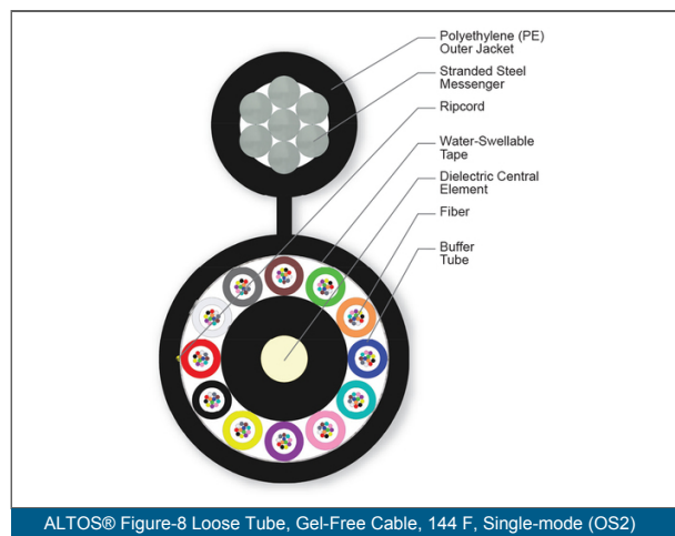
ALTOS® Figure-8 Loose Tube, Gel-Free Cable, 144 F, Single-mode (OS2)
