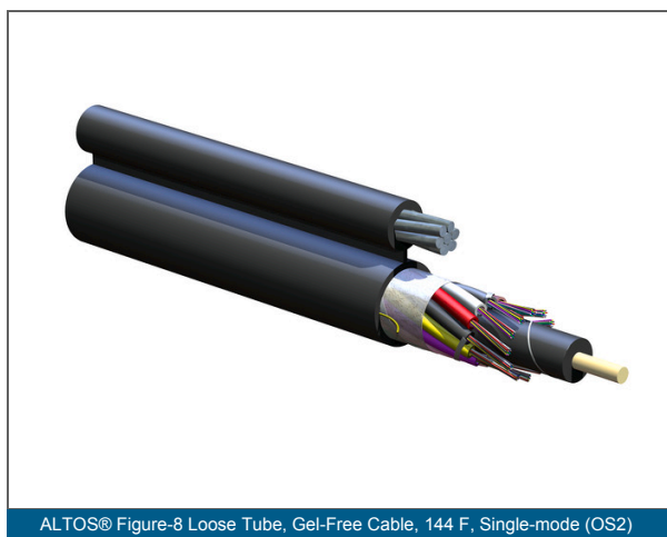
ALTOS® Figure-8 Loose Tube, Gel-Free Cable, 144 F, Single-mode (OS2)
